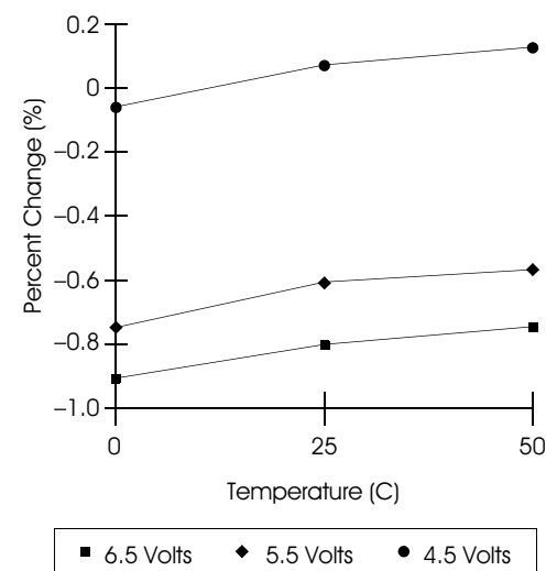
Graph 2-48: Oscillator Stability
