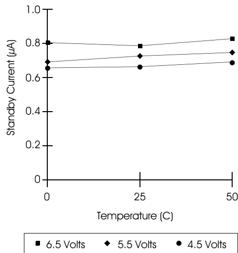
Graph 2-47: Standby Current ( I_{SB} )
