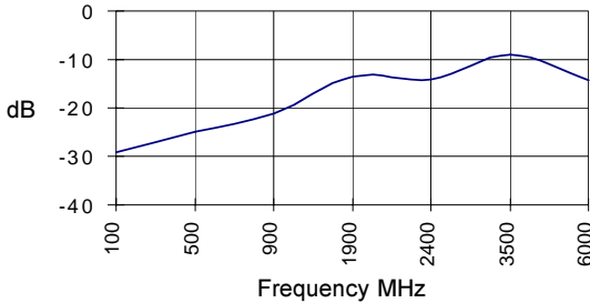
S11, Id =12mA, T=-40C
