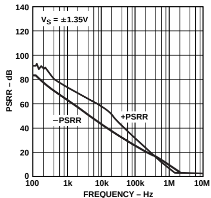
Figure 28. PSRR vs. Frequency at \pm 1.35 V
