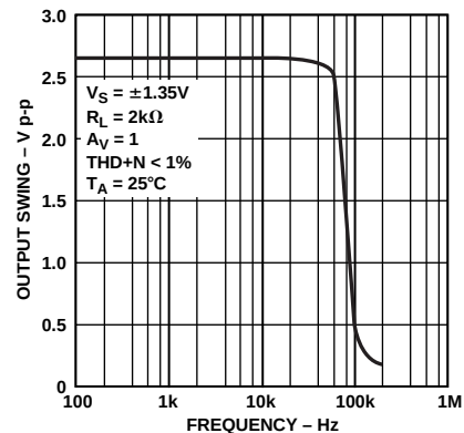
Figure 30. Maximum Output Swing vs. Frequency at 2.7 V
