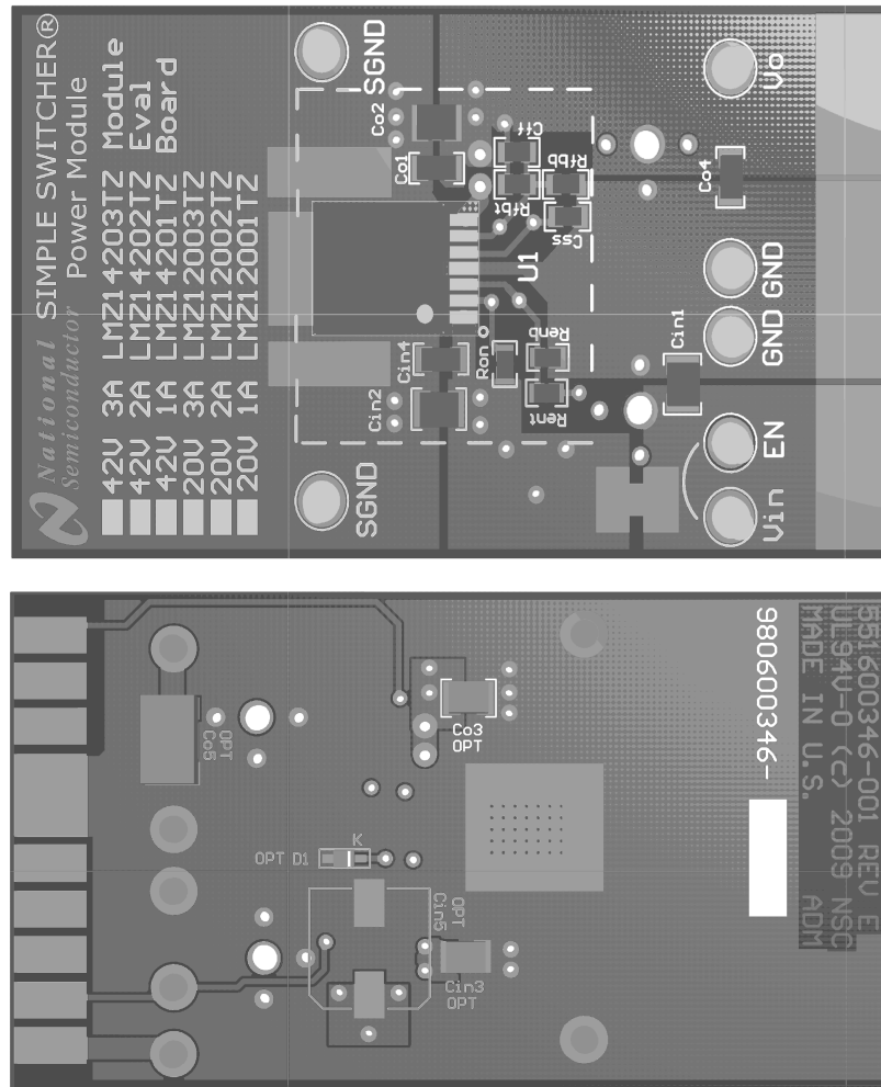
Figure 23. Top And Bottom View Of Evaluation PCB
