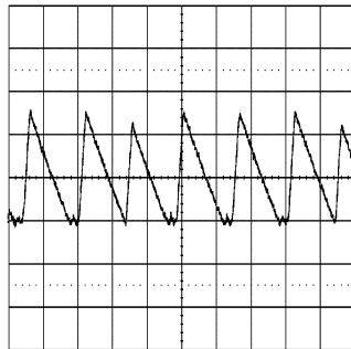
Figure 21. Transition Mode Operation V_{IN} = 12V , V_O = 3.3V , I_O = 0.5 A 2 \mu\text{sec/div}
