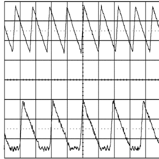
Figure 20. CCM and DCM Operating Modes V_{IN} = 12V , V_O = 3.3V , I_O = 3A/0.4A 2 \mu\text{sec/div}
