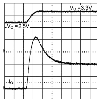
Figure 22. Pre-Biased Startup
