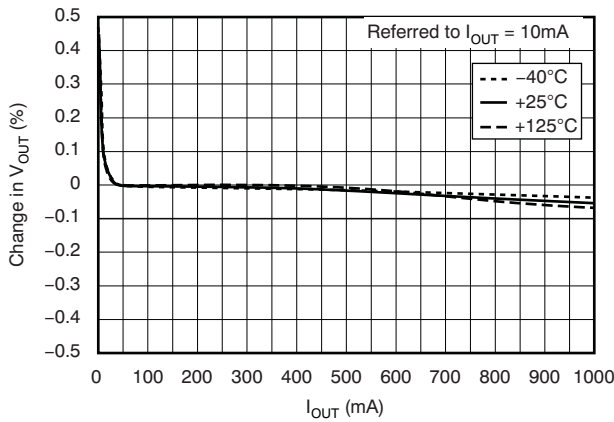
Figure 3. LOAD REGULATION
