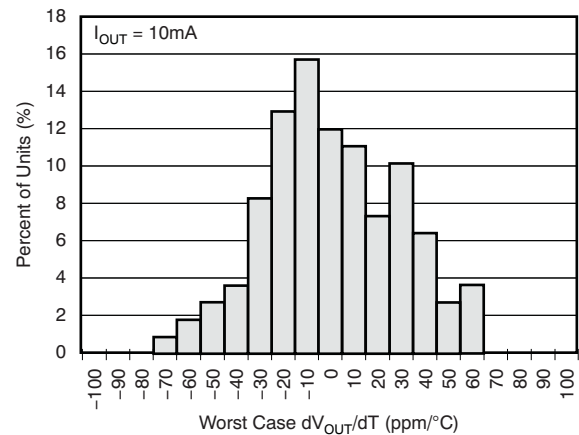
Figure 8. OUTPUT VOLTAGE DRIFT HISTOGRAM
