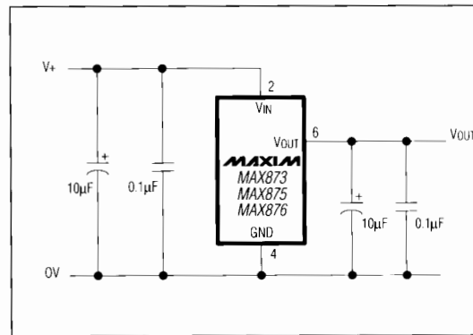
Figure 1. Recommended Bypassing for Good High-Frequency Response
