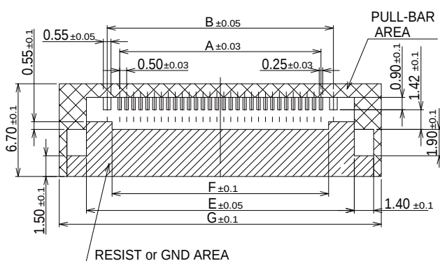
RECOMMENDED FOOTPRINT PATTERN
