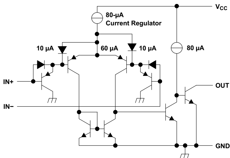
Schematic (Each Comparator)
