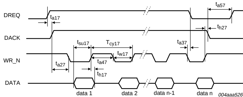
Fig 18. DMA write (multicycle burst).
