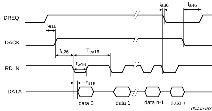
Fig 17. DMA read (multicycle burst).
