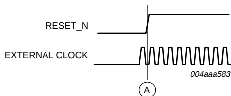
Fig 9. Clock with respect to the external power-on reset.
