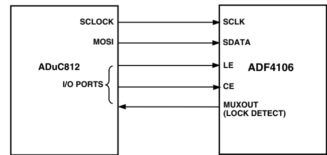
Figure 8. ADuC812 to ADF4106 Interface
