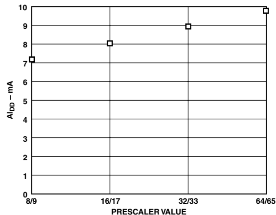
TPC 12. I_{DD} vs. Prescaler Value
