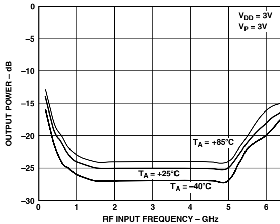
TPC 2. Input Sensitivity
