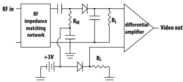
Figure 13. Differential Detector.
