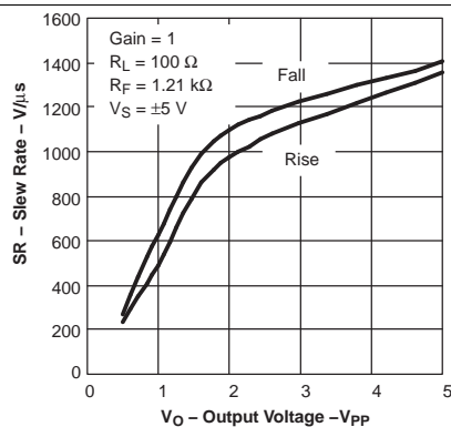
Figure 52. Slew Rate vs Output Voltage Step
