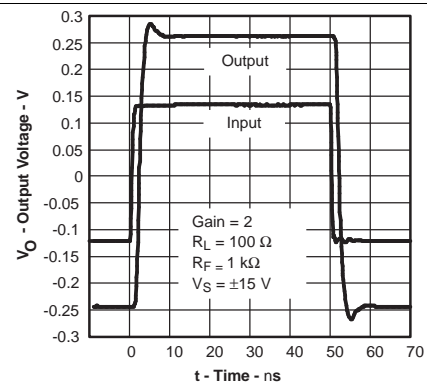
Figure 30. Noninverting Small-Signal Transient Response
