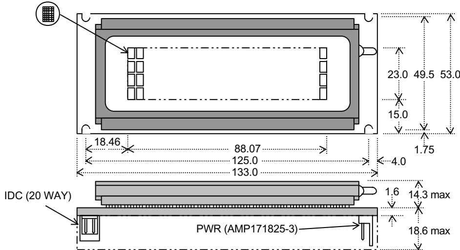
Dimensions in mm & subject to tolerances. Mounting slots 3.5mm dia.
