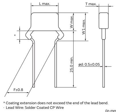
Dimensions code: 0/1/2/3 Lead style code: P1
