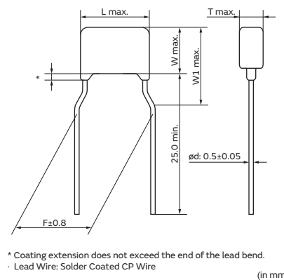
Dimensions code: 2/3/4 Lead style code: K1
