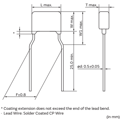
Dimensions code: 0/1 Lead style code: K1
