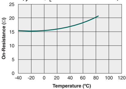
Typical On Resistance vs. Temperature ( I_F=5mA; I_L=100mA Instantaneous)
