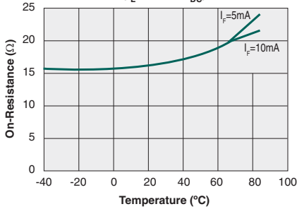
Typical On-Resistance vs. Temperature AC/DC Configuration ( I_L=150mA_{DC} )
