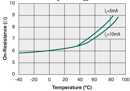
Typical On-Resistance vs. Temperature - DC Configuration ( I_L=150mA_{DC} )
