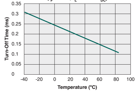
Typical Turn-Off Time vs. Temperature ( I_F=5mA, I_L=100mA_{DC} )
