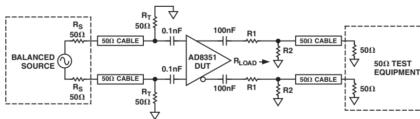
Figure 14. Test Circuit
