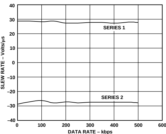
Figure 5. Slew Rate vs. Data Rate
