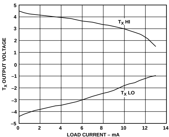
Figure 6. Transmitter Output Voltage vs. Load Current
