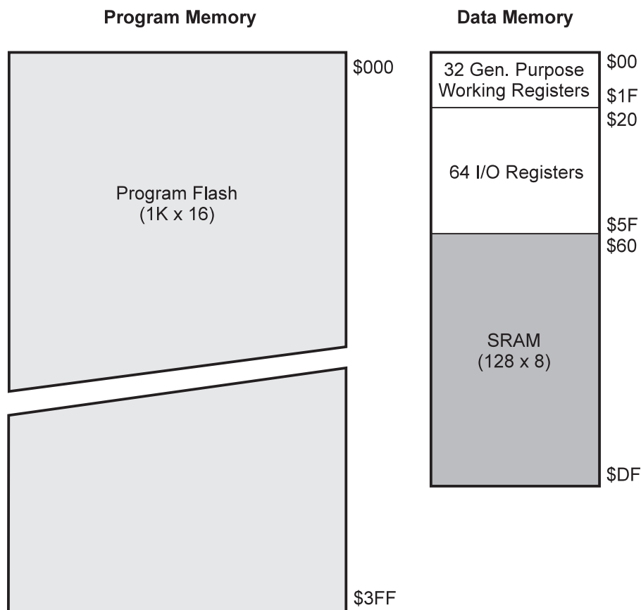
Figure 5. Memory Maps
