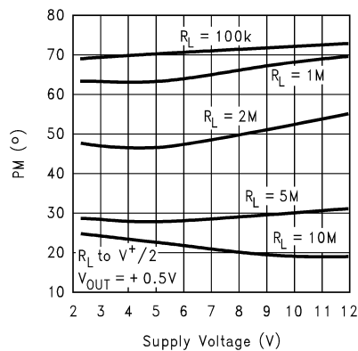
Phase Margin (Worst Case) vs Supply Voltage
