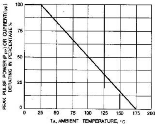
Fig. 2-PULSE DERATING CURVE
