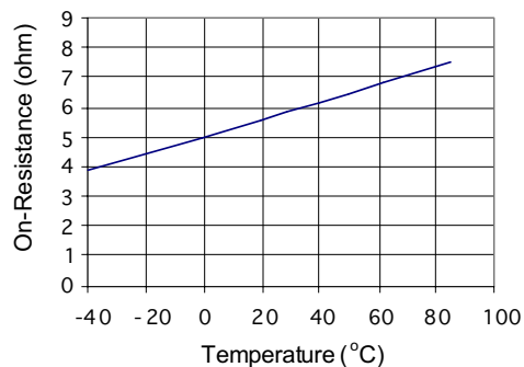
Form B_Typical On-Resistance vs. Temperature (Load Current= 170mA; I F =0mA)
