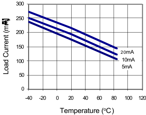
Figure 1. Form A_Typical Load Current vs. Temperature
