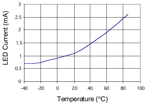
Form A_Typical I_F for Switch Dropout vs. Temperature (Load Current=170mA)
