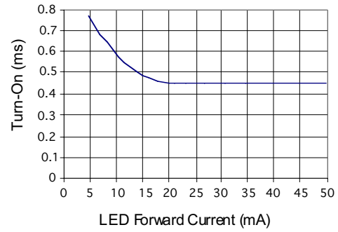
Form A_Typical Turn-On vs. LED Forward Current (Load Current=170mA)
