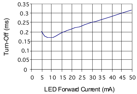
Form A_Typical Turn-Off vs. LED Forward Current (Load Current=170mA)
