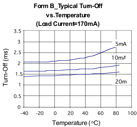
Figure 11. Form B_Typical Turn-Off vs. Temperature (Load Current = 170 mA)
