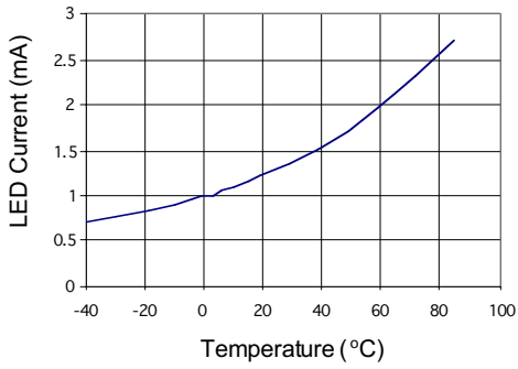
Form A_Typical I_F for Switch Operation vs. Temperature (Load Current=170mA)
