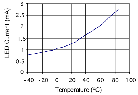
Form B_Typical I_F for Switch Operation vs. Temperature (Load Current=170mA)
