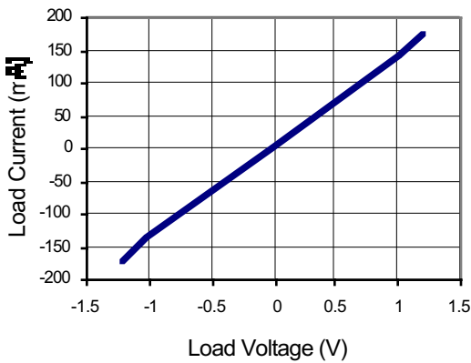
Figure 2. Form A_Typical Load Current vs. Load Voltage (Ambient Temp.= 25°C; I_F=5\text{ mA} )
