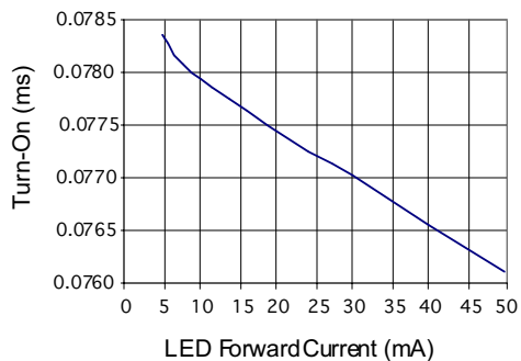
Form B_Typical Turn-On vs. LED Forward Current (Load Current=170mA)
