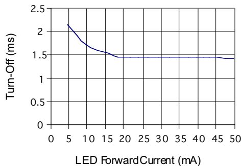
Form B_Typical Turn-Off vs. LED Forward Current (Load Current=170mA)
