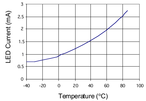
Form B_Typical I_F for Switch Dropout vs. Temperature (Load Current=170mA)
