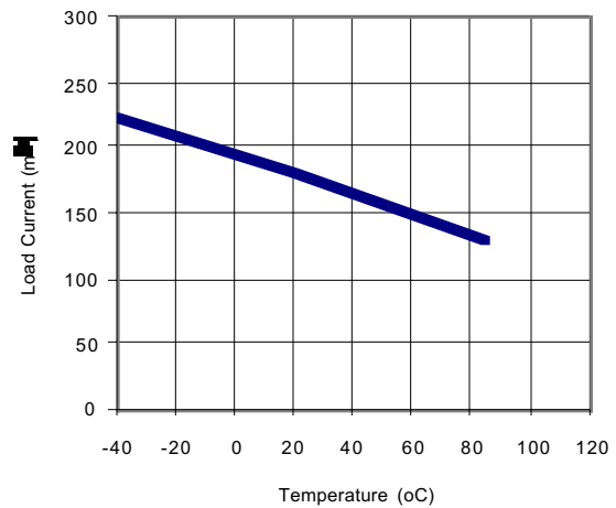
Figure 4. Form B_Typical Load Current vs. Temperature
