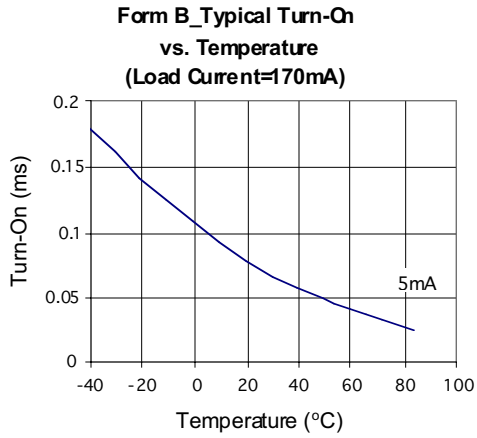
Figure 10. Form B_Typical Turn-On vs. Temperature (Load Current = 170 mA)
