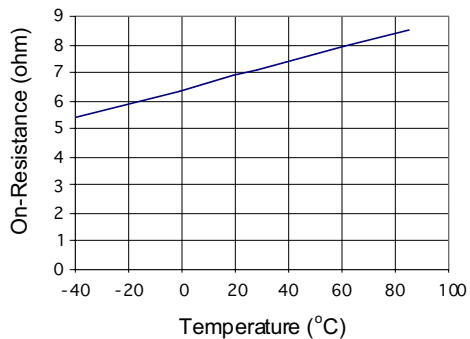
Form A_Typical On-Resistance vs. Temperature (Load Current= 170mA; I F =5mA)
