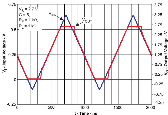
Figure 6. Output Overdrive Recovery
