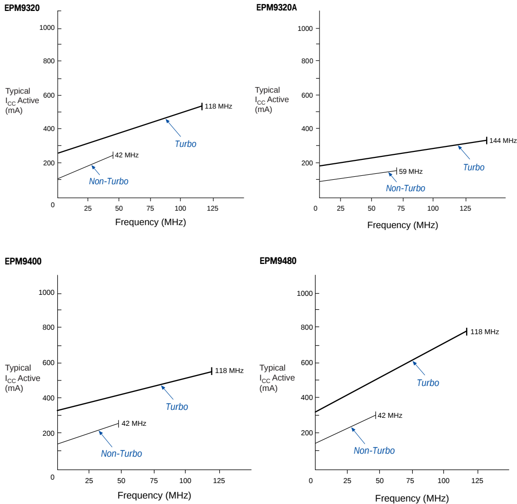
Figure 15. I_{CC} vs. Frequency for MAX 9000 Devices (Part 1 of 2)
