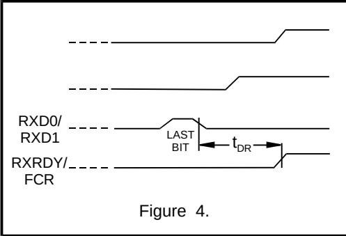
RECEIVER OPERATION
