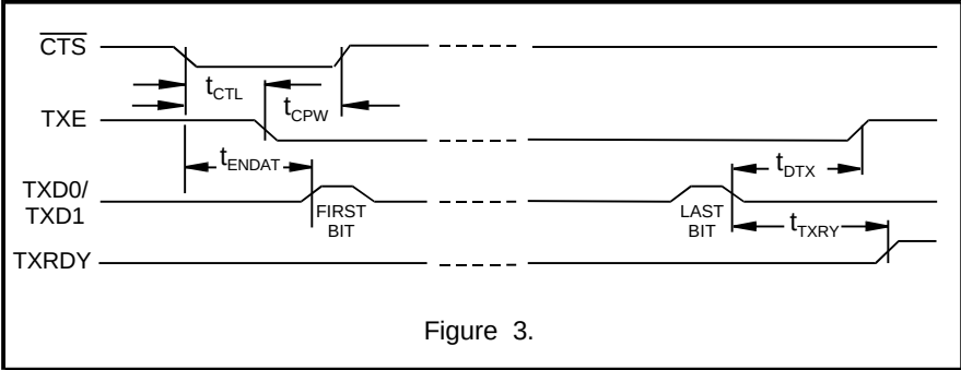
TRANSMITTER OPERATION
