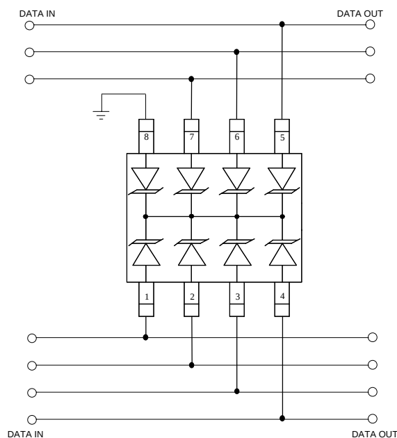
Connection Diagram
