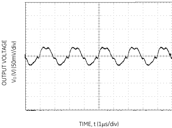
Figure 33. Typical output ripple and noise (Co=2x47µF ceramic, VIN = 12V, Io = Io,max.).
