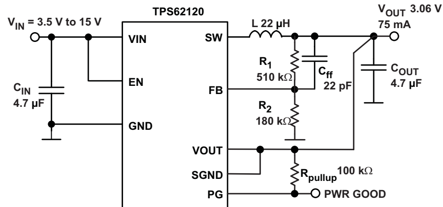
Figure 38. TPS62120 3.06-V Output Voltage Configuration
