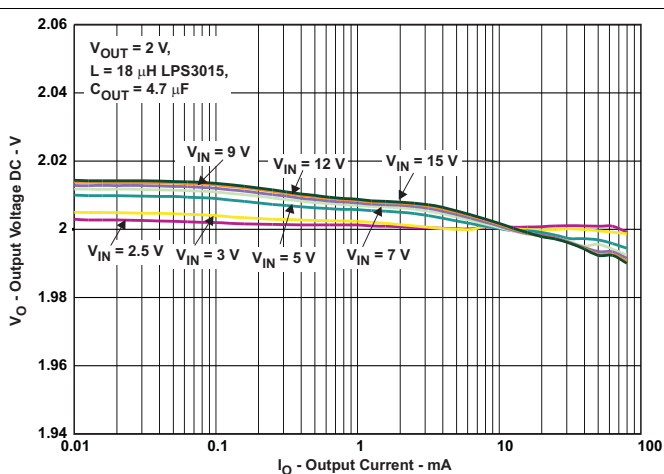
Figure 19. 2.0-V Output Voltage DC Regulation
