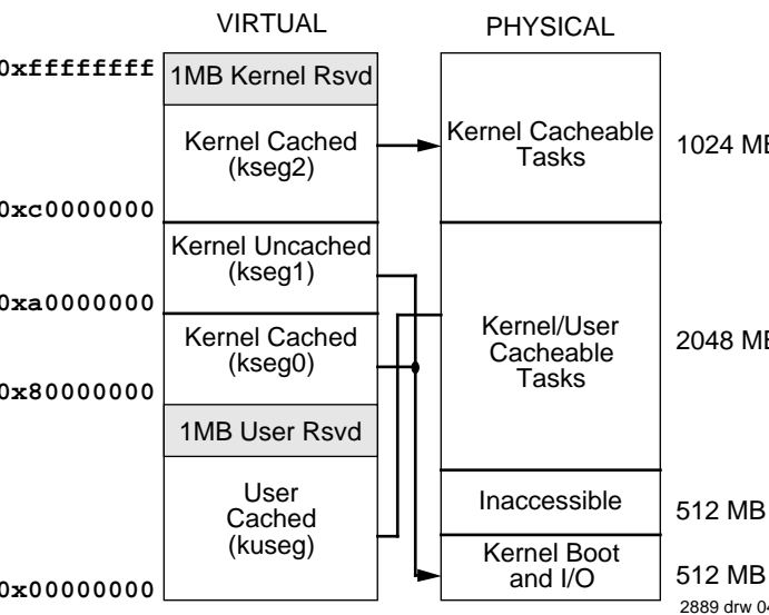
Figure 4. Virtual to Physical Mapping of Base Architecture Versions
