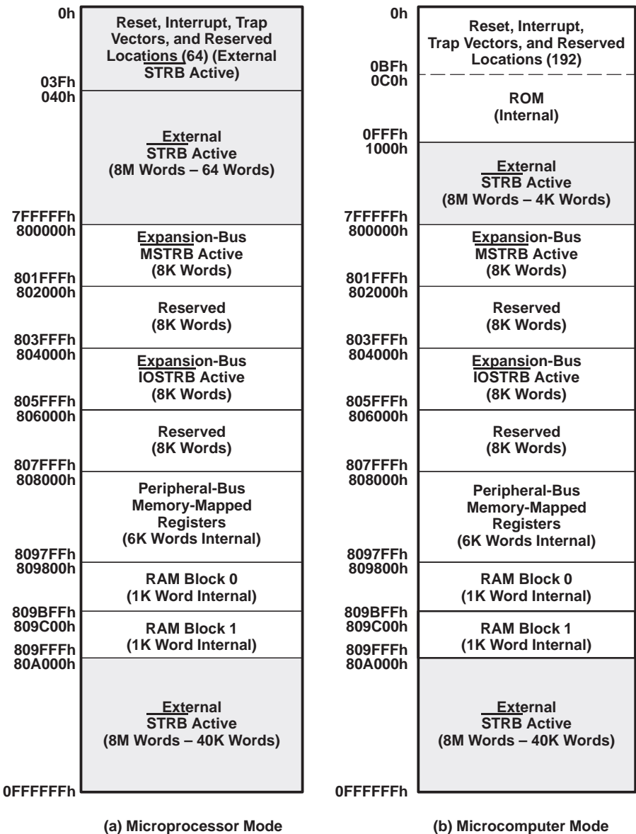
Figure 1. Memory Map
