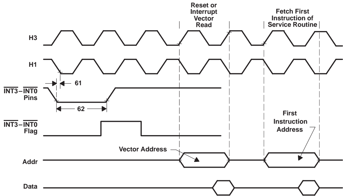
Figure 21. Timing for \overline{\text{INT3}}\text{--}\overline{\text{INT0}} Response [ Q = t_{\text{c(H)}} ]
