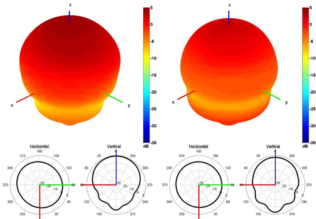
1176 AND 1575 MHz Radiation pattern
