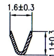
B-B SECTION
