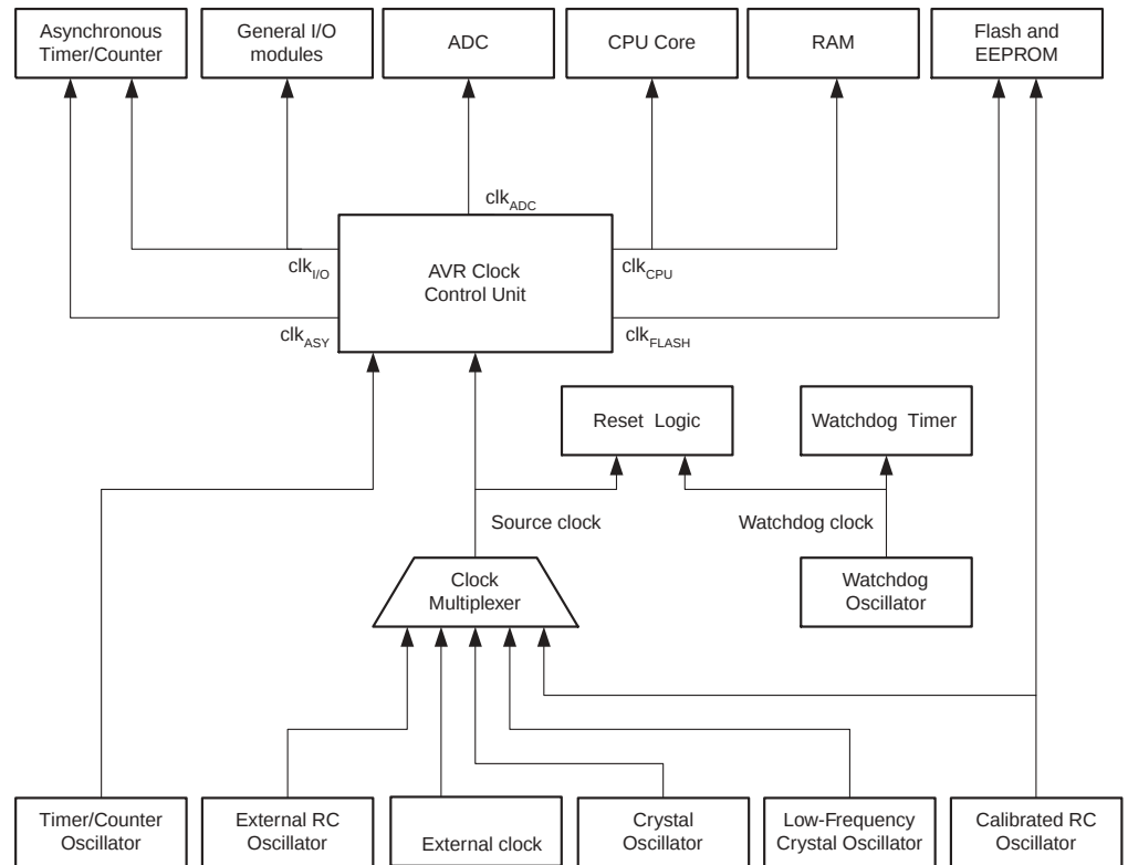
Figure 18. Clock Distribution
