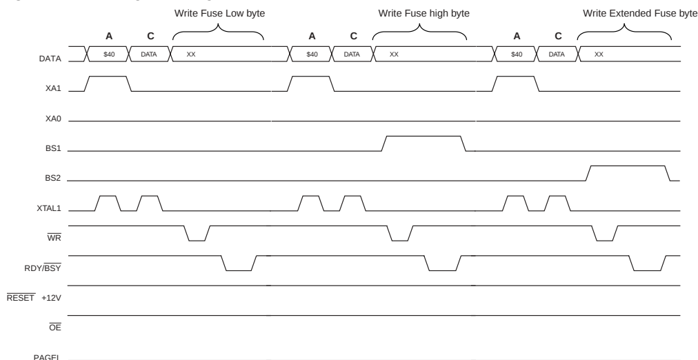
Figure 139. Programming the Fuses
