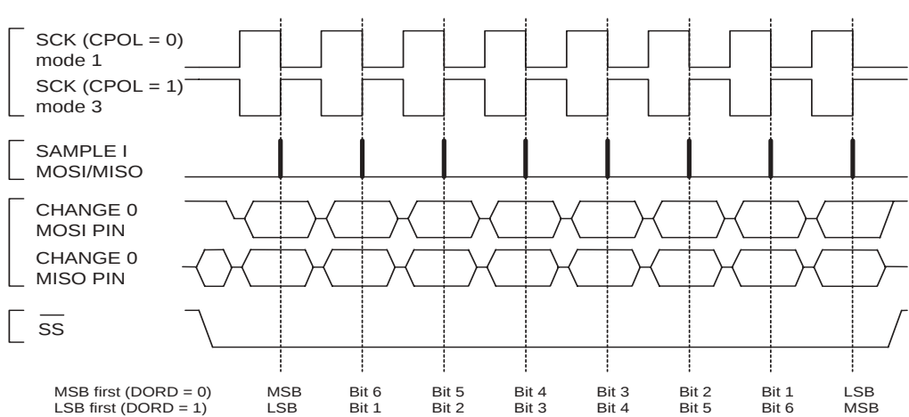
Figure 78. SPI Transfer Format with CPHA = 1
