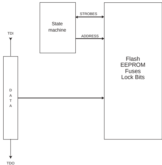
Figure 150. Virtual Flash Page Load Register
