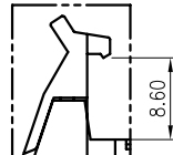
STANDARD LATCH
