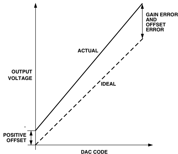
Figure 3. Positive Offset Error and Gain Error
