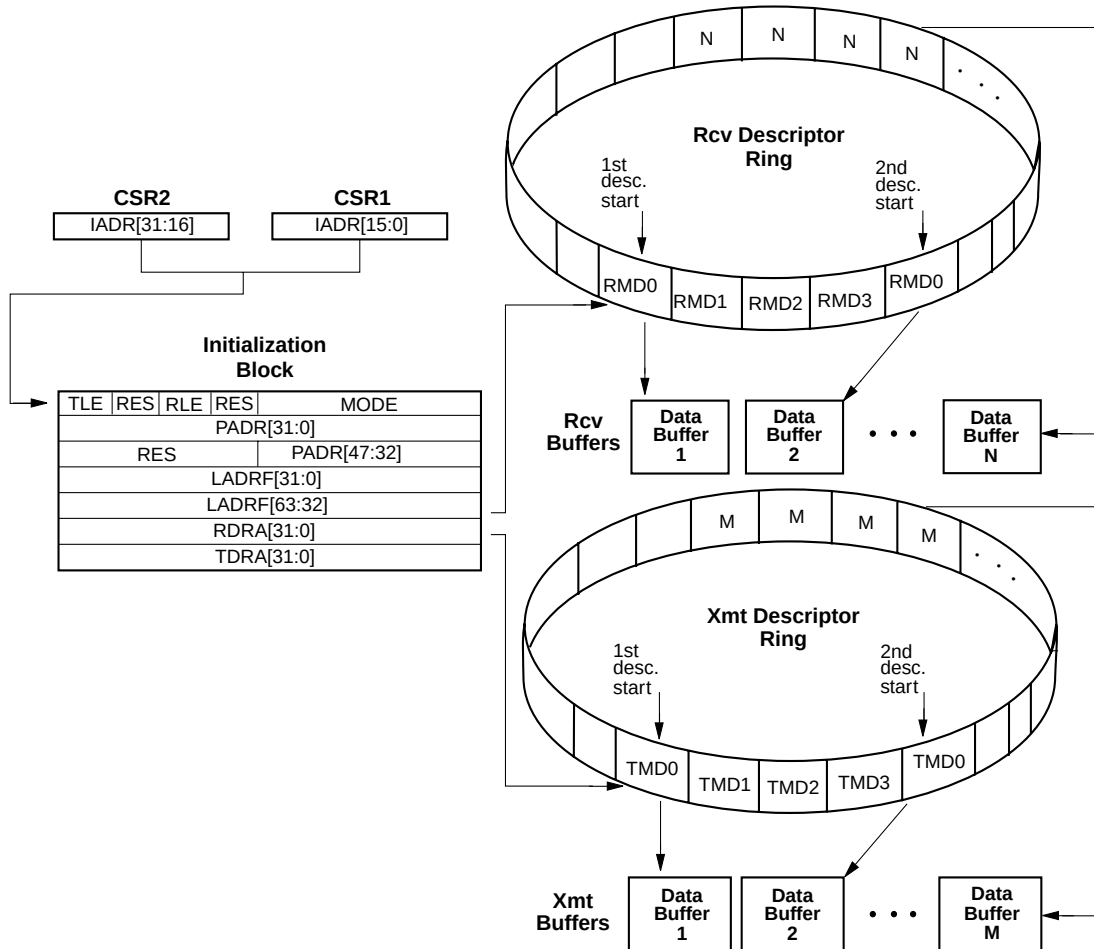
Figure 29. 32-Bit Software Model
