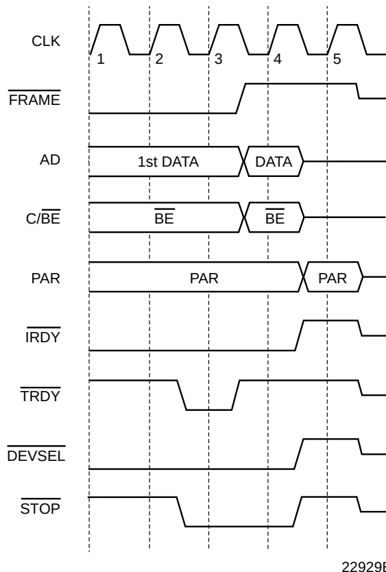
Figure 6. Disconnect Of Slave Burst Transfer - No Host Wait States
