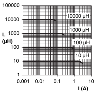
Typical L vs Current
