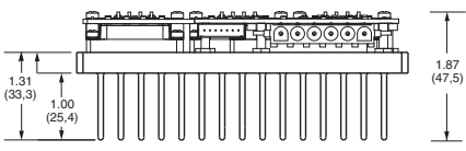
1" Fin Option Fin spacing and relief are the same for both Fin options.
