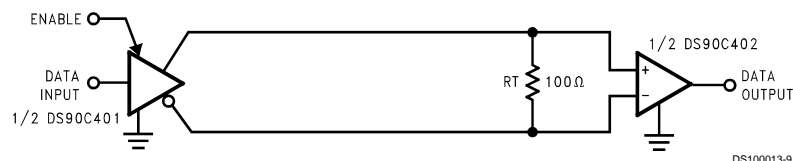
FIGURE 4. Point-to-Point Application
